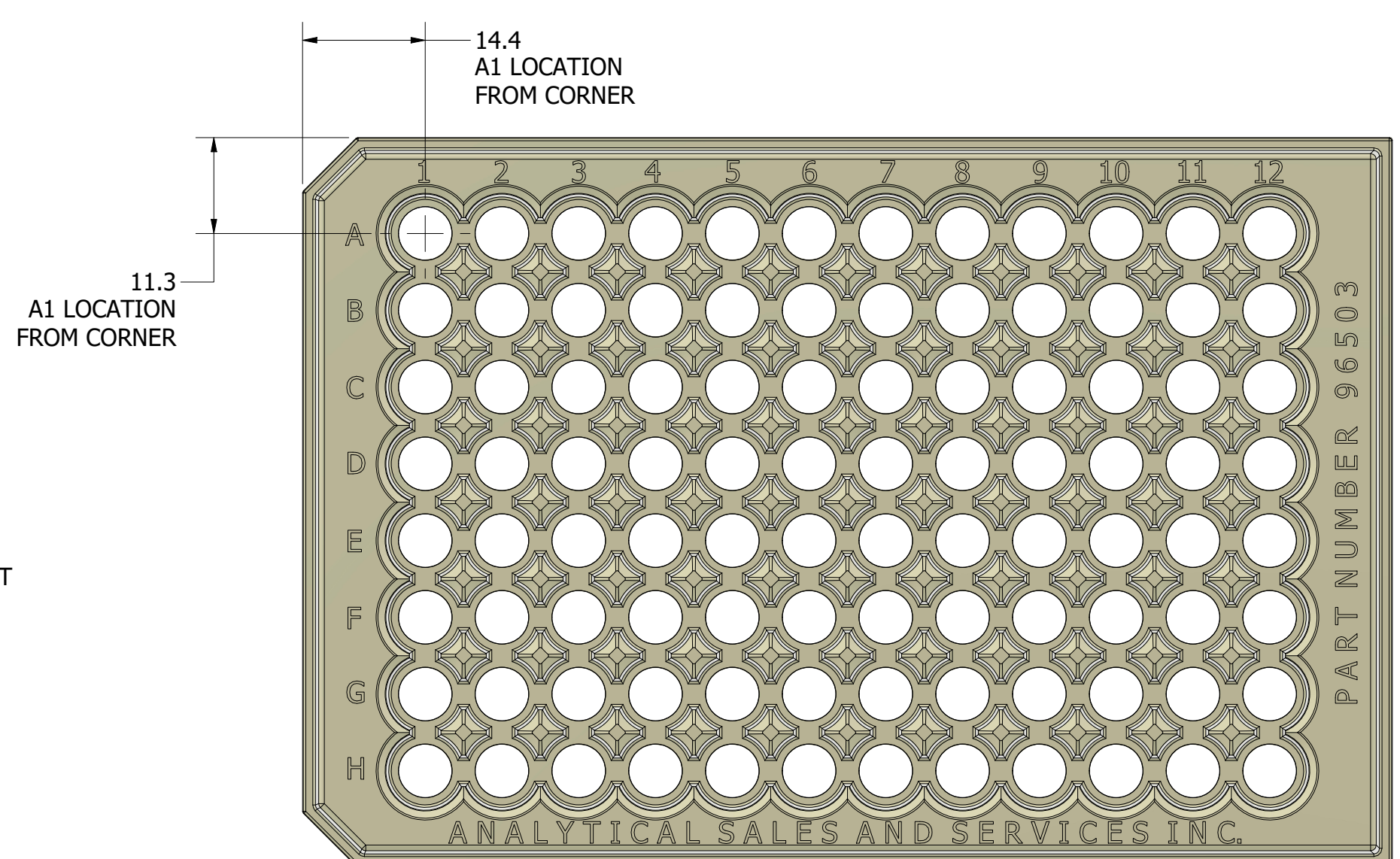
VIAL TRAY TOP VIEW (WITHOUT LID)
