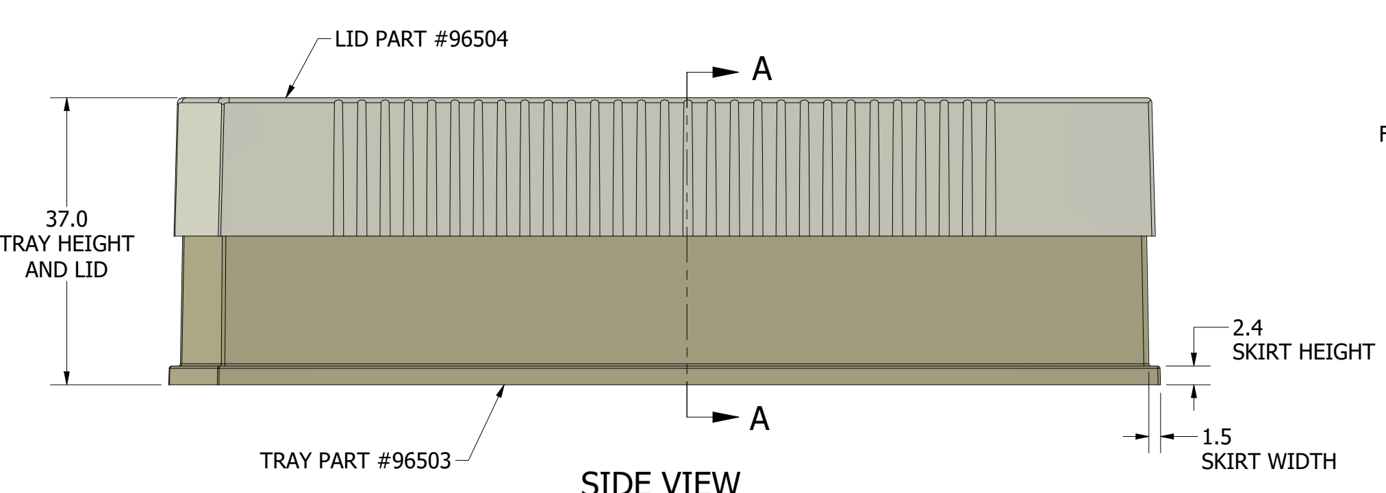
SIDE VIEW
