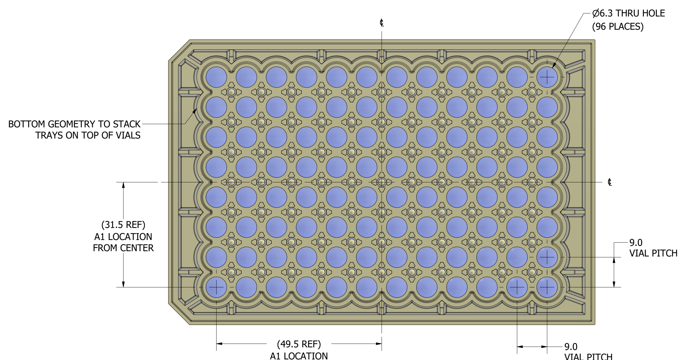
BOTTOM VIEW
